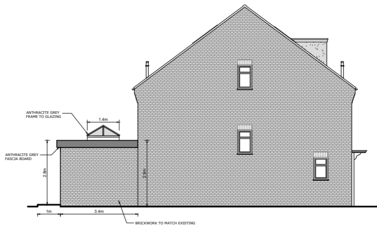
REAR ELEVATION SCALE 1:100
